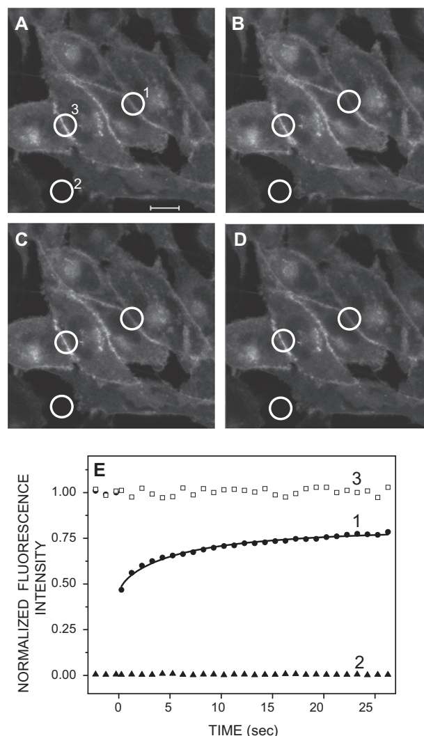
Fig. 2. Representative images of fluorescence recovery after photobleaching of 5-HT 1A R-EYFP. Fluorescence images of CHO-5-HT 1A R-EYFP cells represent confocal sections of the cell periphery acquired at room temperature (~23 °C). Panels A–D show fluorescence intensity monitored at various time points corresponding to pre-bleach, bleach, immediate post-bleach and complete recovery, respectively. Panel E shows a representative plot for the normalized fluorescence intensity of 5-HT 1A R-EYFP (●) corresponding to region 1, and the normalized background intensity (▲), corresponding to region 2. The normalized fluorescence intensity in a control region 3 (□) monitored for the same time period, indicates no significant photobleaching due to repeated scanning. The dimensions of the regions are only representative. The scale bar represents 10 μm. See Section 2 for other details. Taken from Ref. [24].
