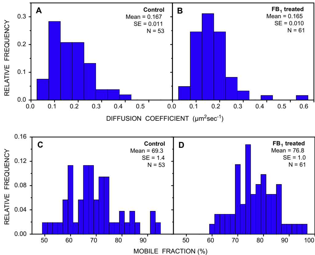
Fig. 3. Frequency distribution histograms of diffusion coefficient and mobile fraction of 5-HT 1A R-EYFP. The frequency distribution histograms are obtained by fitting the normalized recovery of individual experiments. The histograms for diffusion coefficients (panels A and B) and mobile fraction (panels C and D) for control (untreated) cells, and FB 1 -treated cells, respectively, are shown. The means \pm standard errors are shown in all cases. N represents the number of independent experiments performed in each case. See Section 2 and Table 1 for other details.
