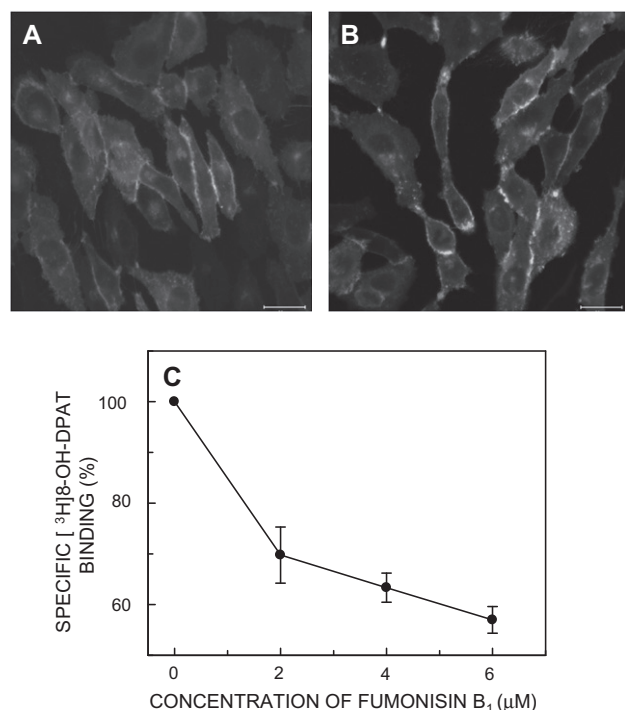
Fig. 1. Cellular morphology and the overall distribution of 5-HT 1A R-EYFP remain unaltered in control and cells treated with 6 μM FB 1 . Typical fluorescence distribution of 5-HT 1A R-EYFP in CHO-5-HT 1A R-EYFP cells is shown under (A) control and (B) FB 1 -treated conditions. Fluorescence images of cells grown on coverslips and placed in Biopetechs FCS2 closed chamber system were acquired at 37 °C in presence of HEPES-Hanks buffer. The scale bar represents 20 μm. Panel C shows the loss of specific agonist binding of the human serotonin 1A receptor upon FB 1 treatment. Adapted and modified from Ref. [17].
